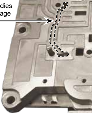
Transfer Plate
