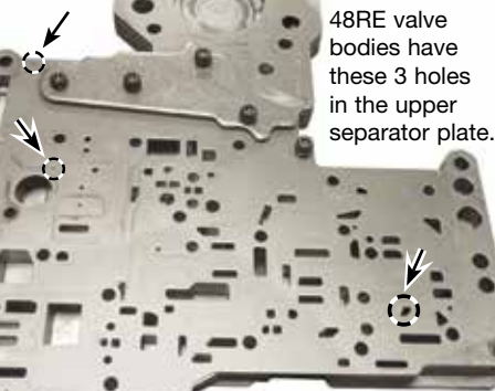
Upper Separator Plate
